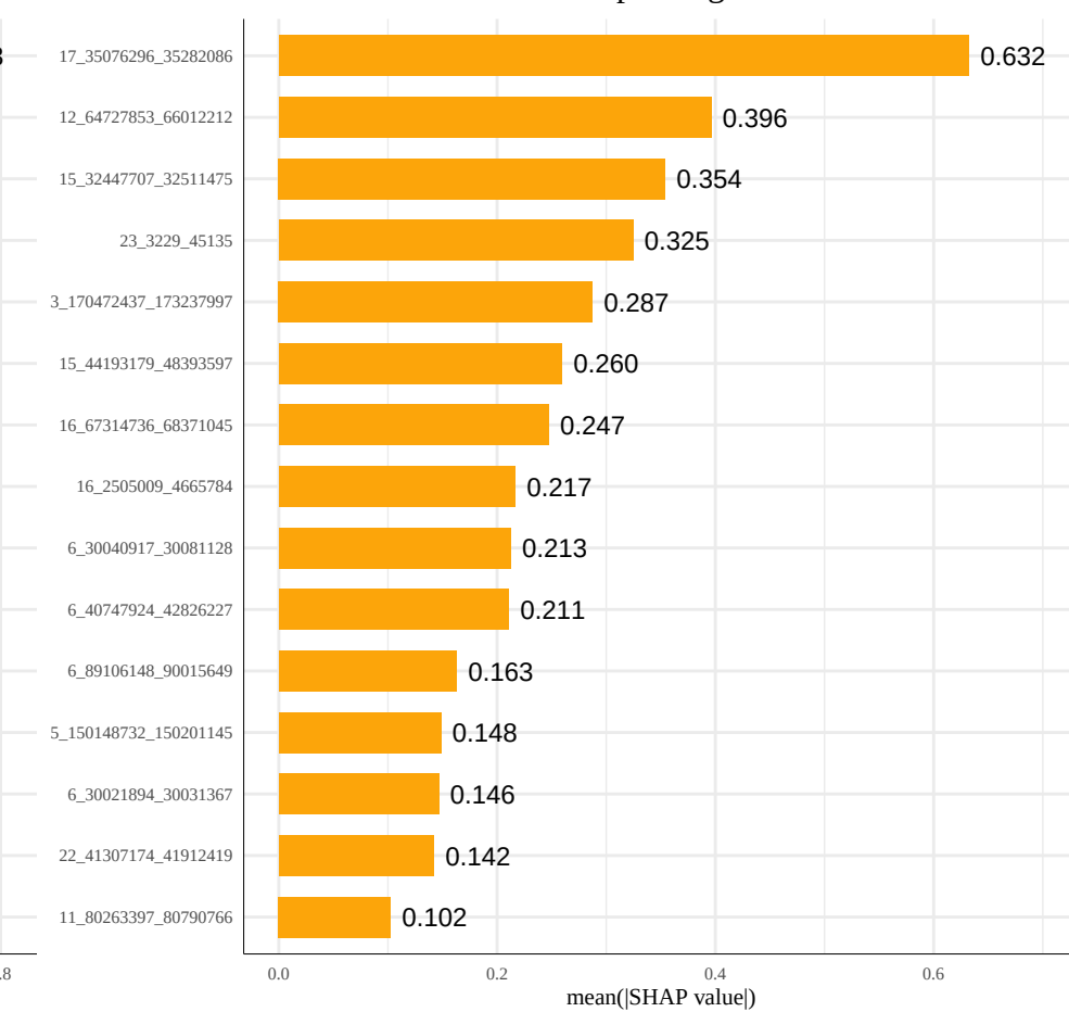
C SHAP Values for Class Triple Neg Prediction
